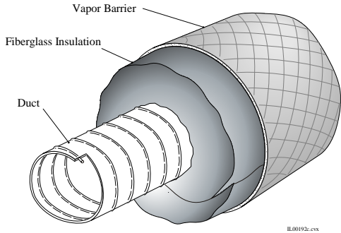
Figure 3. Typical duct construction
